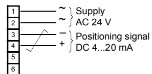
ZM121/A (DC 4...20 mA oder DC 0...20 V Phs)
