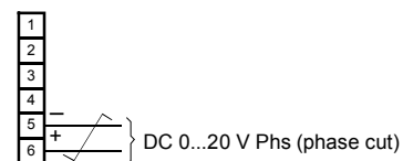
ZM121/A (DC 4...20 mA oder DC 0...20 V Phs)
